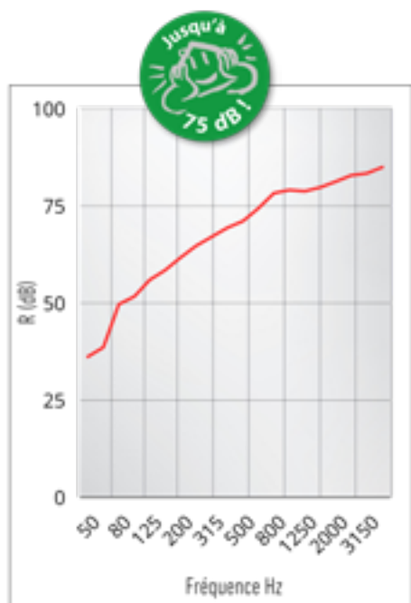
Acoustix Pan-terre fibro-plâtre Test AC 0245 | AC-21-058-06 Cloison double ossature métallique R_w (C; C_{tr}) = 75 (-2; -7) \text{ dB}
